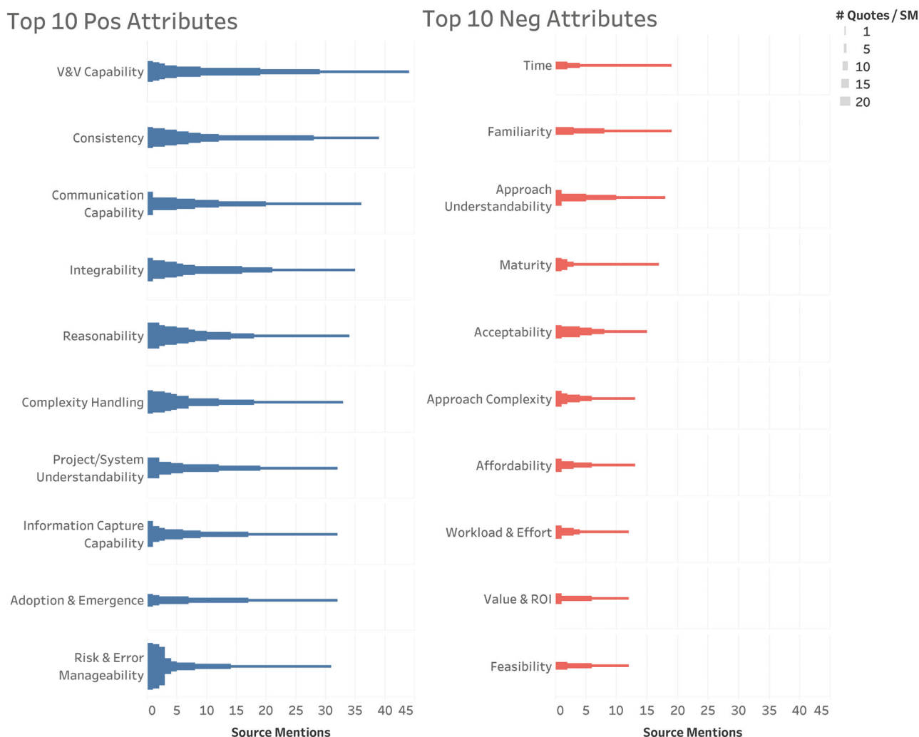
FIGURE 5 Top ten most positively used attributes (left) and top ten most negatively used attributes (right) sorted by source mentions
