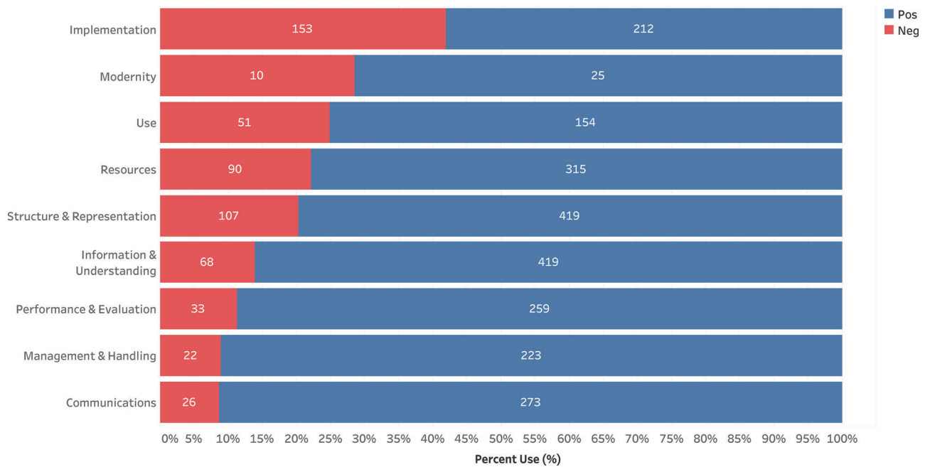
FIGURE 3 Attribute categories by descending negative percentage use
