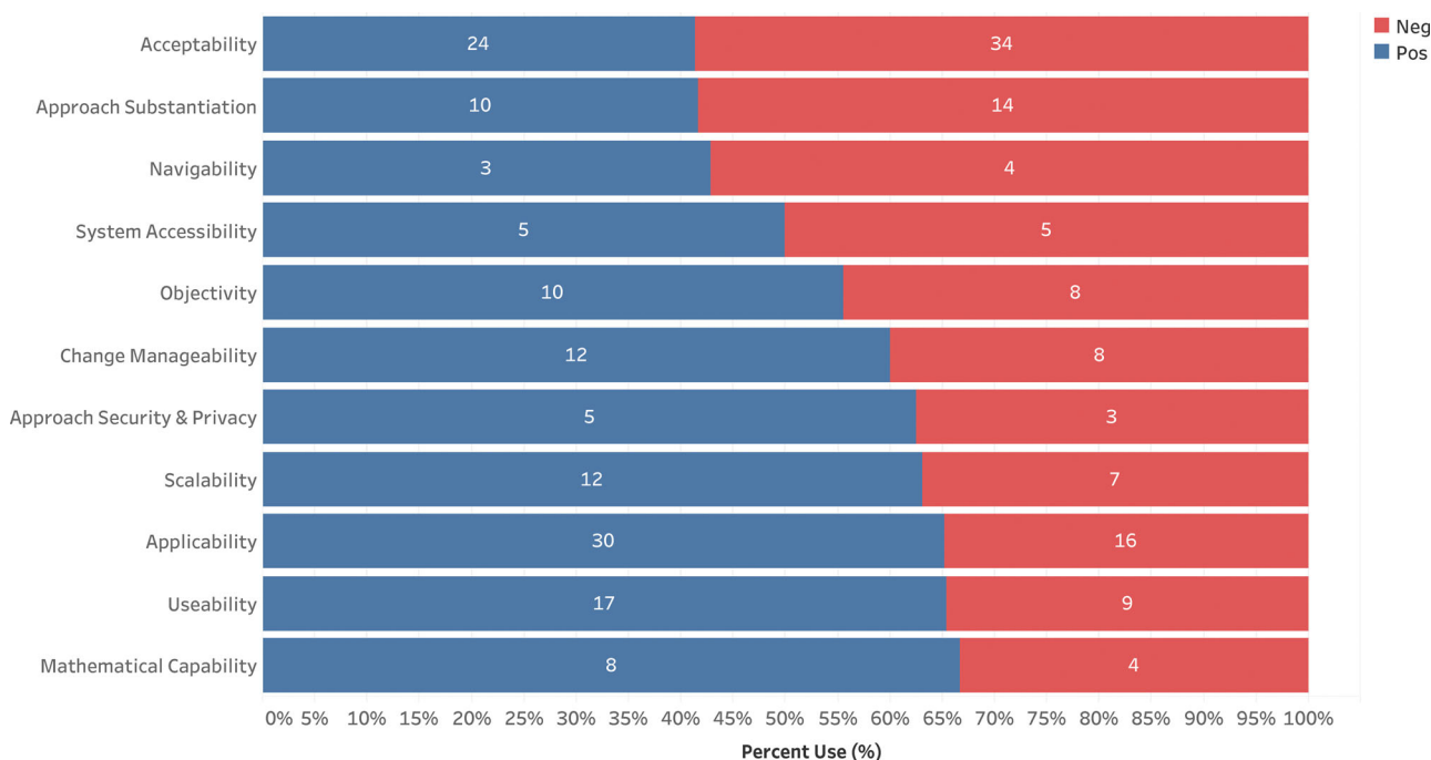
FIGURE 6 Distribution of mixed-perception attributes by descending positive percentage of uses
