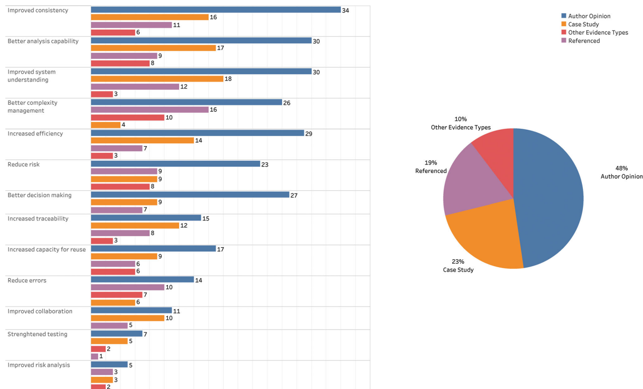
FIGURE 8 INCOSE-, IBM-, and OMG-promoted benefits evidence distribution (left). Overall evidence distribution for INCOSE-, IBM-, and OMG-promoted benefits by percentage
