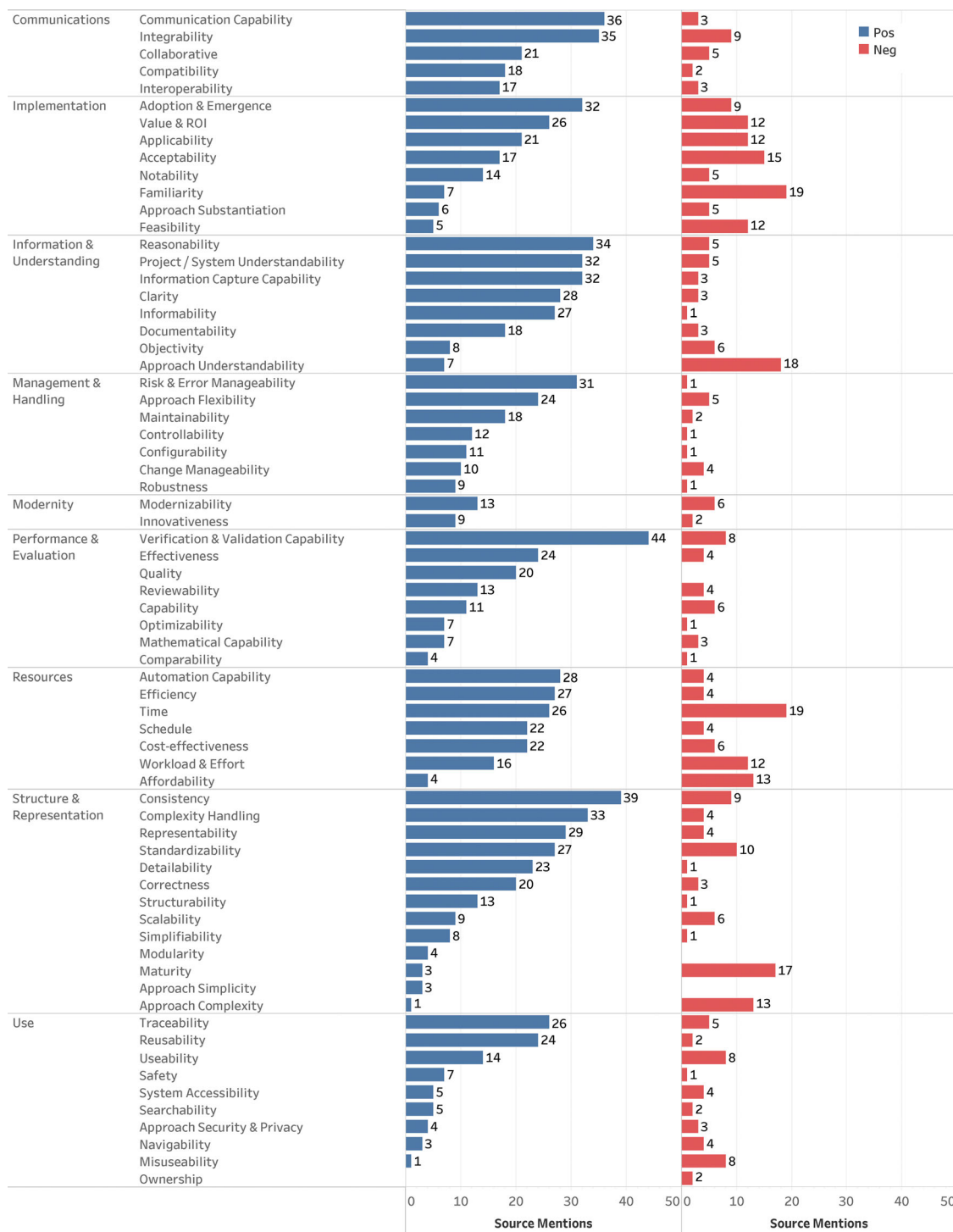
FIGURE 4 Attribute categories with individual attributes sorted by descending positive uses by number of source mentions
